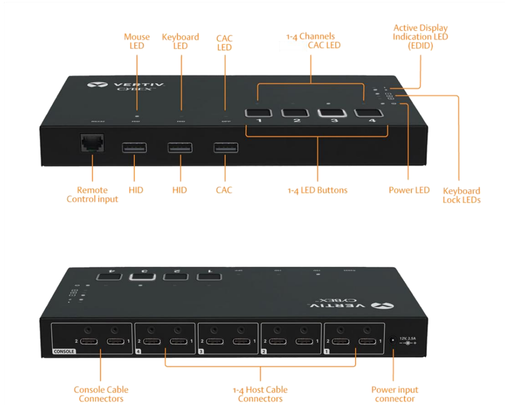
Figure 3 – 4PT DH Micro Switch Device (SC945SFF)
