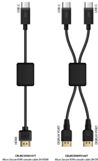
Figure 6 – Console Cables
