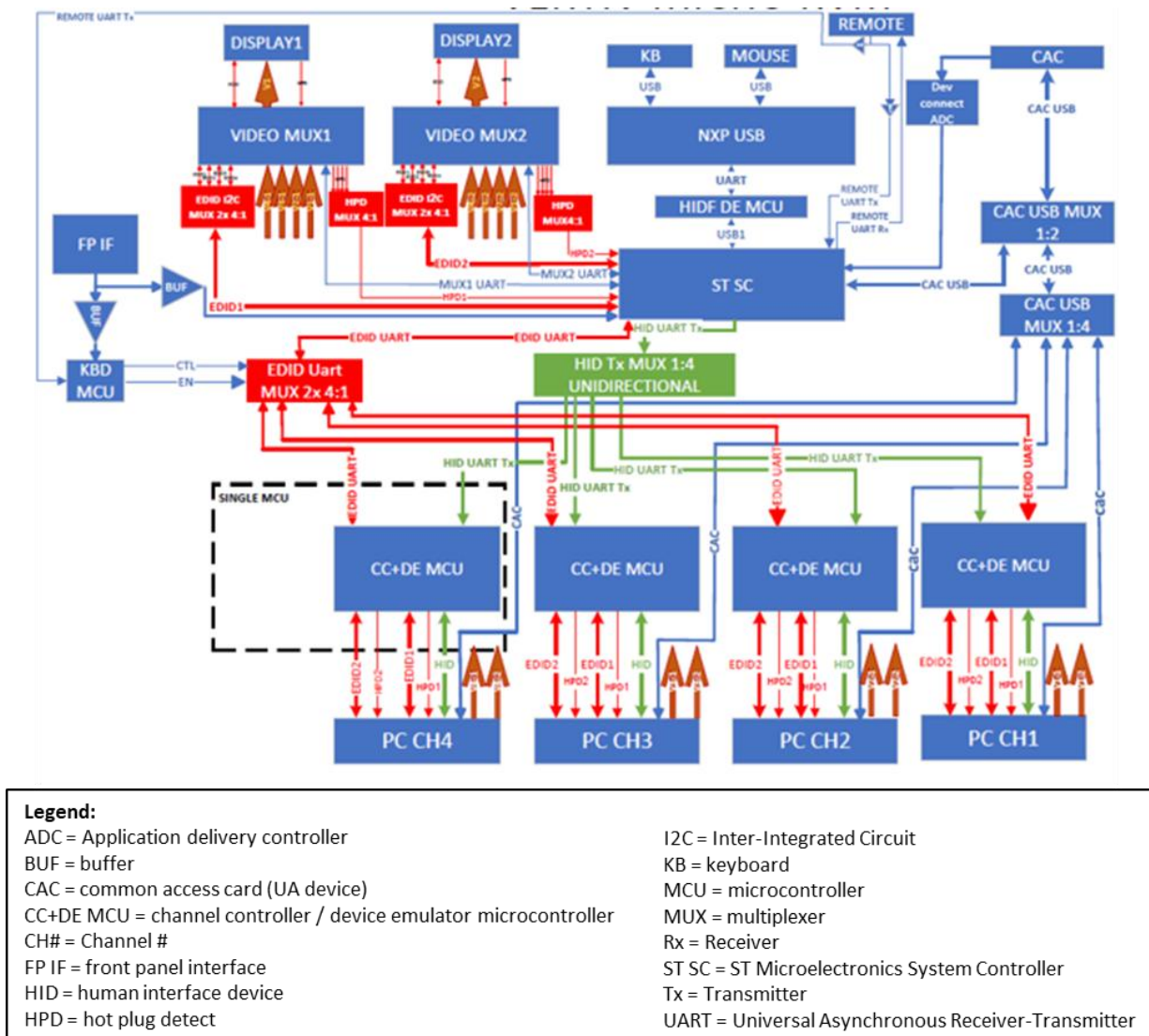
Figure 9 – Detailed block diagram of KVM Switches
