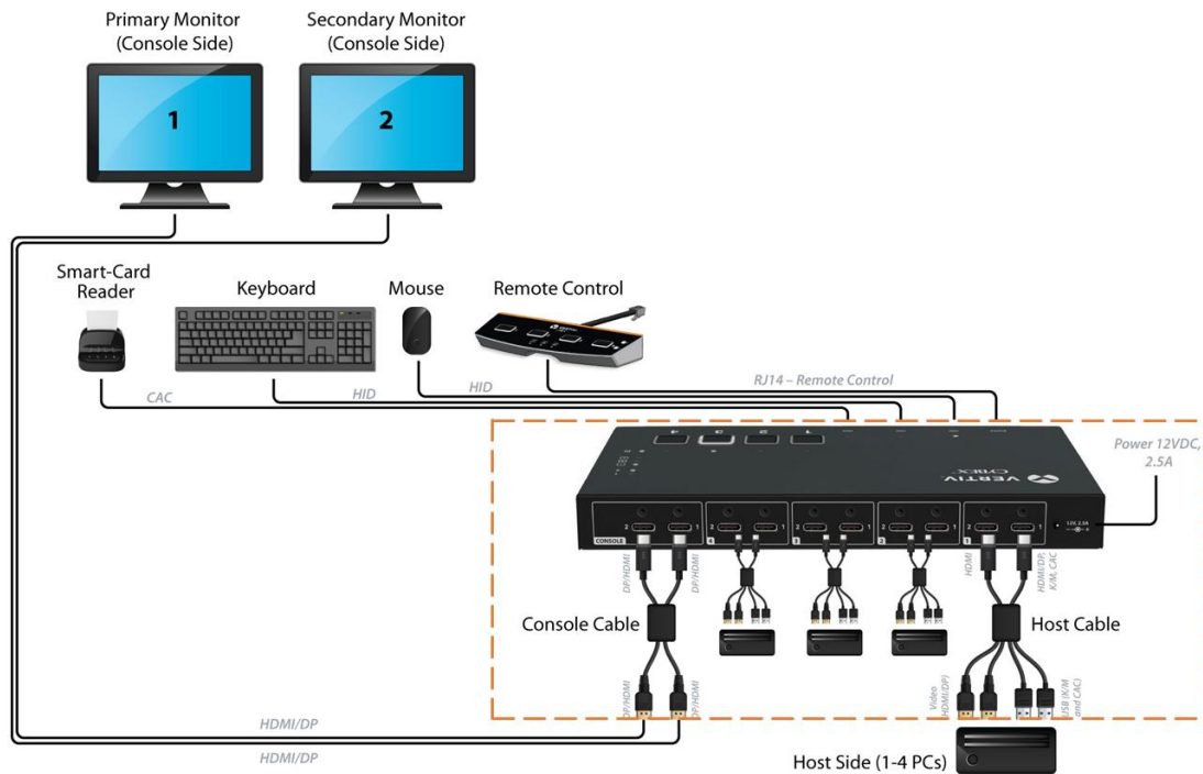
Figure 1 – Switch Evaluated Configuration
