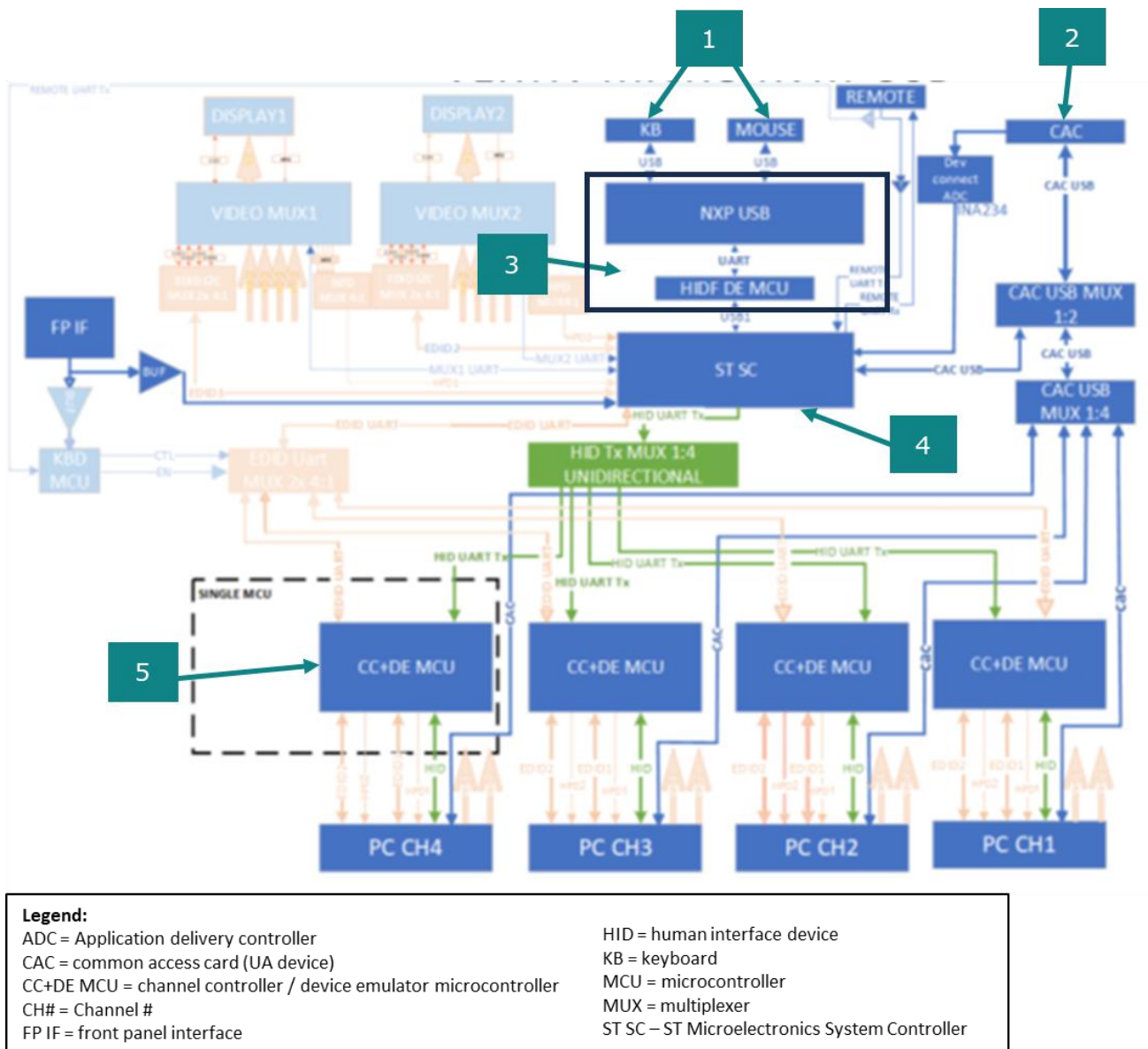
Figure 7 – Detailed block diagram of KVM USB switching functionality
