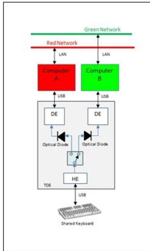
Figure 8 – Simplified Switching Diagram
