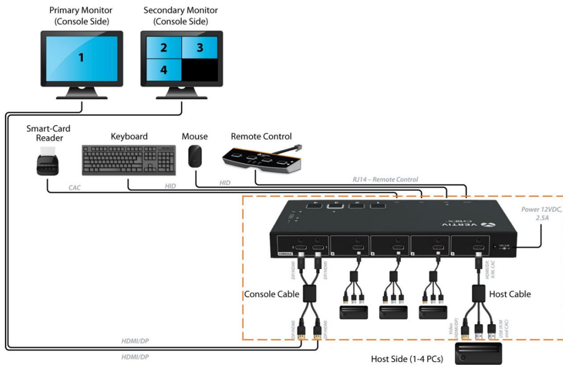
Figure 2 – Multi-Viewer Evaluated Configuration
